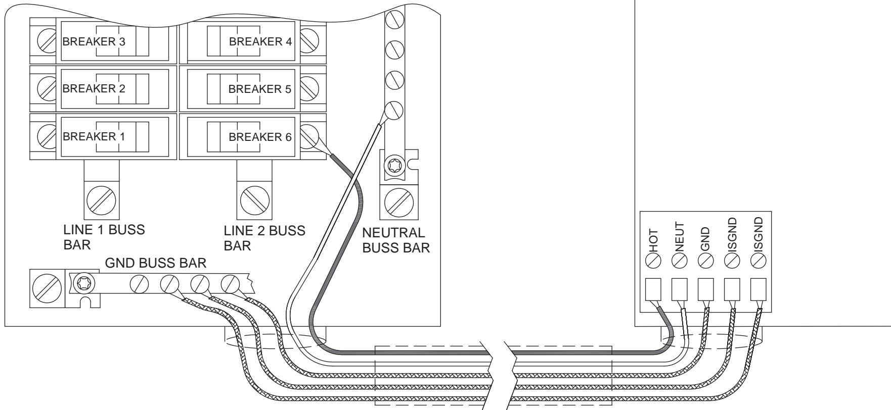
PARTIAL VIEW OF LC2000/TMS CONSOLE
